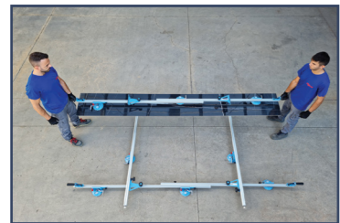
Traversi smontabili per lastre strette Dismantable cross bar for narrow slabs
